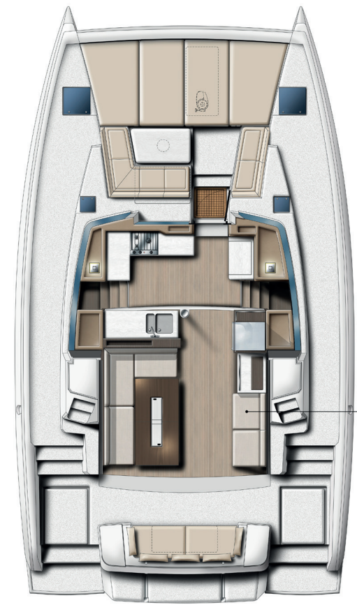
COCKPITS AND SALOON
