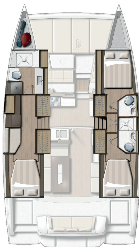
3 DOUBLE CABINS / 3 HEADS / 2 SHOWERS VERSION VERSION 3 CABINES DOUBLES / 3 SDB / 2 DOUCHES
