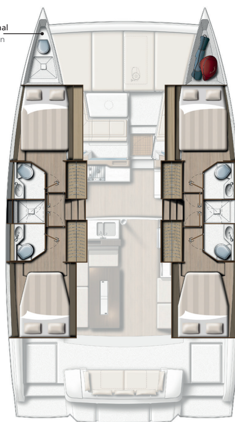
4 DOUBLE CABINS / 4 HEADS / 2 SHOWERS VERSION VERSION 3 CABINES DOUBLES / 3 SDB / 2 DOUCHES
