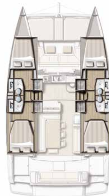
Version 4 cabines / 4 sdb 4 cabins and 4 baths version
